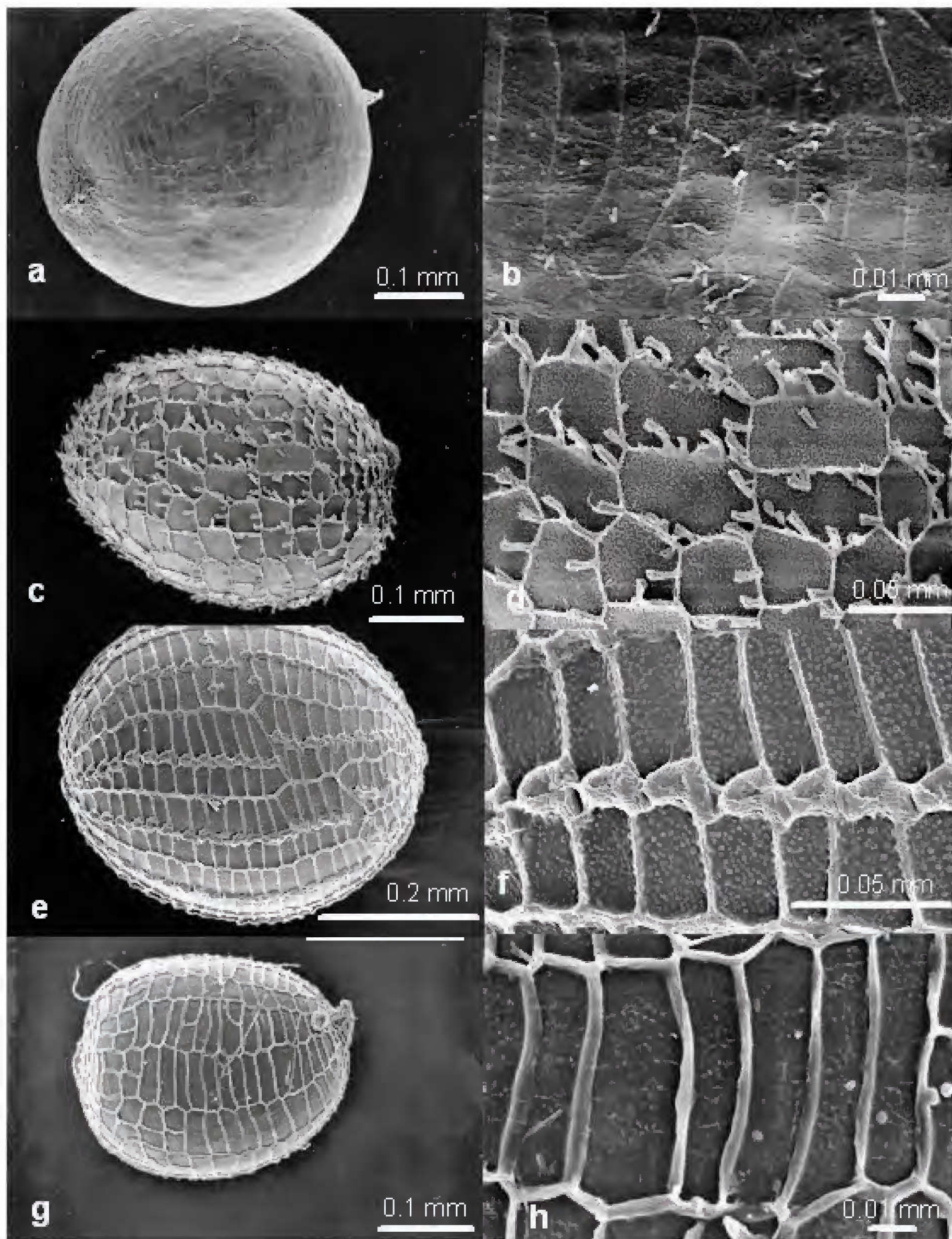
Fig. 8. Seed and seed surface: Eriocaulon rivicola a, b ; E. scariosum c, d ; E. schultzii e, f ; E. scullionii g, h . (a-b from George 12635; c-d from Wilson 989; e-f from Fensham 956; g-h from Leach 2566).
